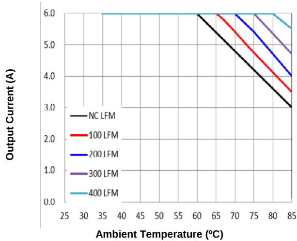
Figure 7. Current Derating Curve for Airflow Direction 3 (Ref. Fig. 8 for Airflow Direction; typical Vin, open frame, soldered interface)
