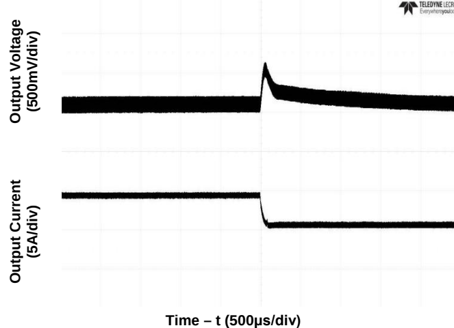
Figure 6. Transient Load Response (typical Vin, load current steps from 50% to 75% at a slew rate 0.1A/µs)
