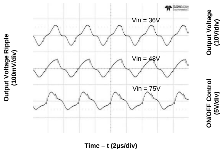
Figure 3. Output Ripple Voltage at Full Load
