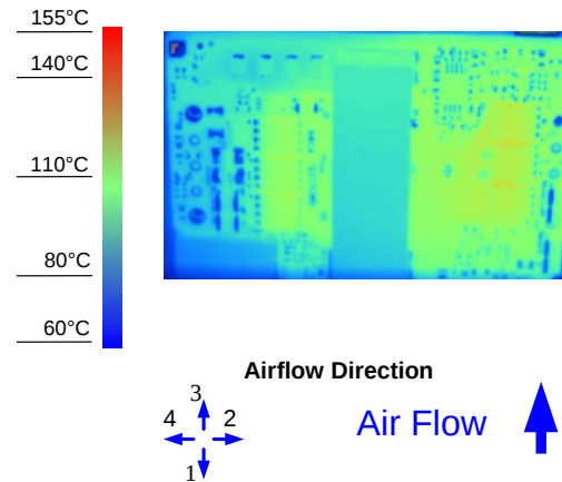
Figure 8. Thermal Image for Airflow Direction 3 (11.3A output, 55°C ambient, 200 LFM, typical Vin, open frame, soldered interface)
